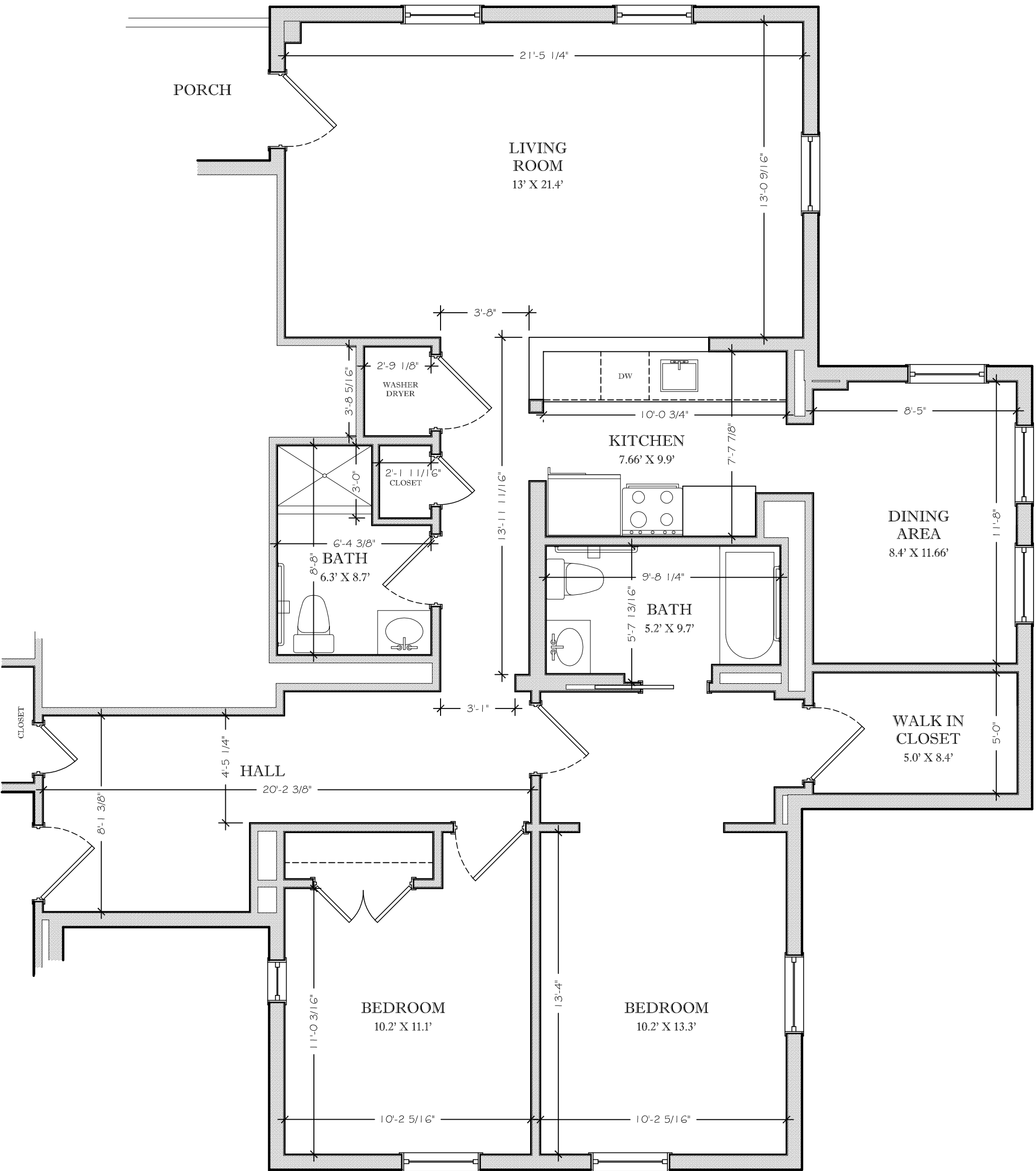
1 UNIT #192 - JOHN BLDG. SCALE 1/4"=1'-0"
